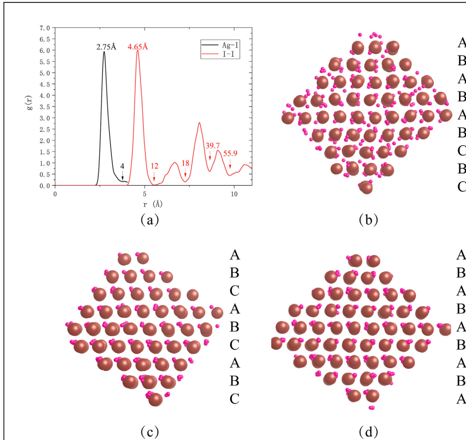
Fig. 11. The RDF (a) and structure (b) at about 480 K after cooling from \alpha -AgI at 700 K. The structures of \gamma -AgI (c) with fcc iodine sublattice and \beta -AgI (d) with hcp iodine sublattice at about 480 K is also demonstrated for comparison purposes.
