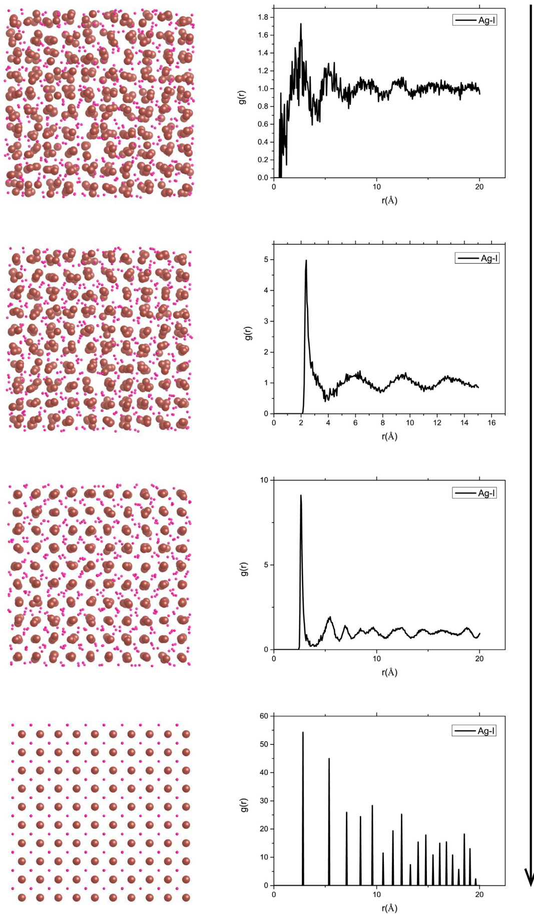
Fig. 6. Snapshots of the configurations during the transition from disordered to ordered \gamma -AgI. The corresponding RDF is also shown.
