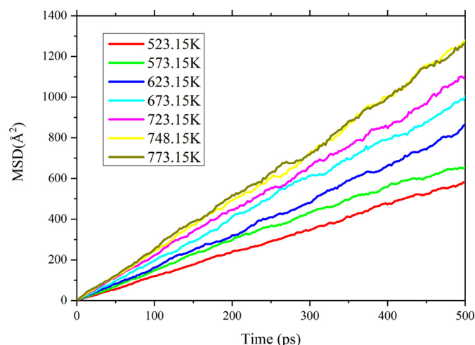
Fig. 8. Mean-squared displacement of \text{Ag}^+ at different temperatures from 525.15 K to 773.15 K.
