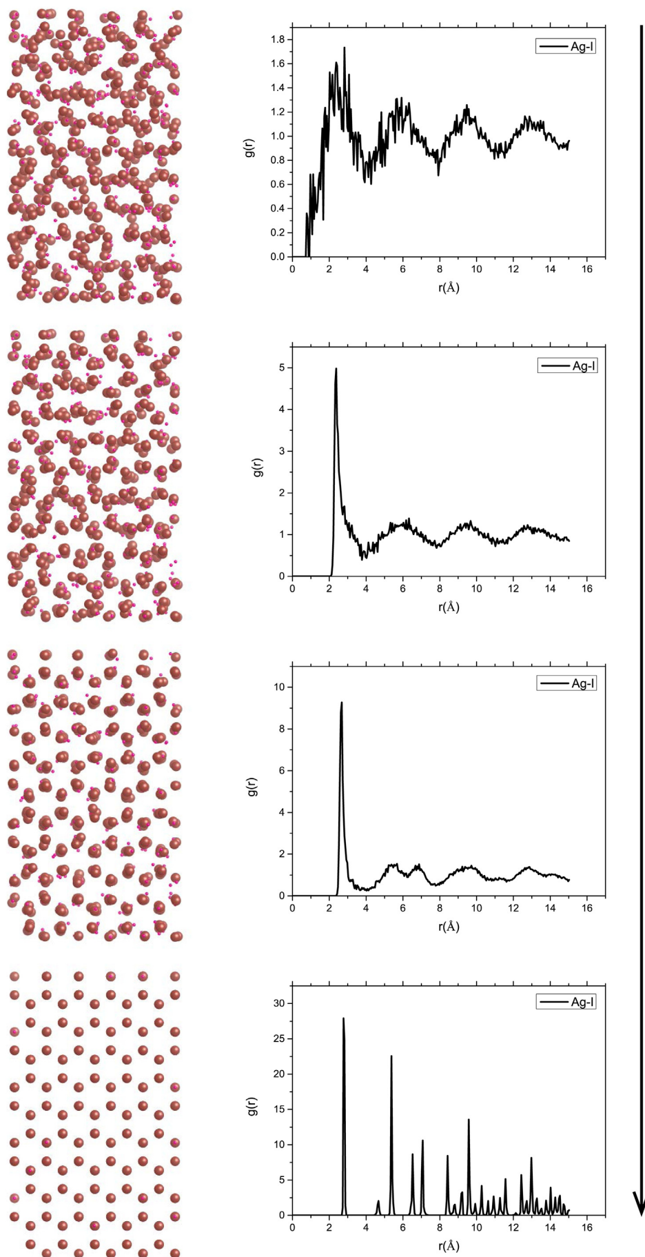
Fig. 5. Snapshots of the configurations during the transition from disordered to ordered \beta -AgI. The corresponding RDF is also shown.
