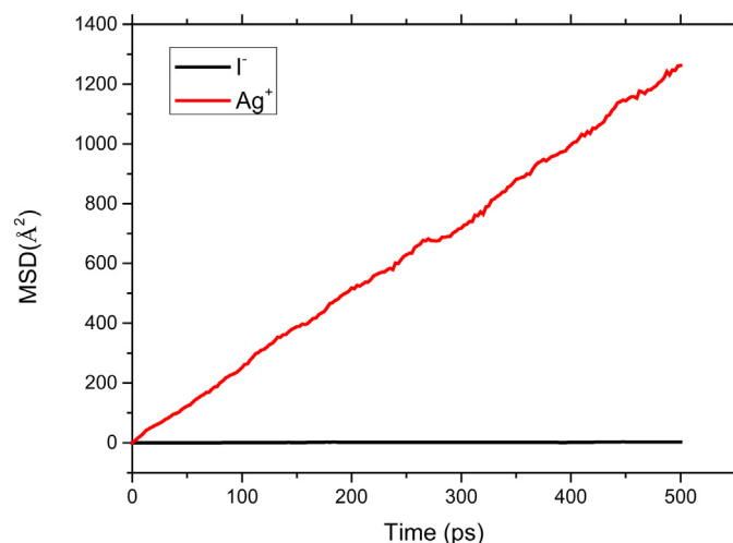
Fig. 7. Mean-squared displacement of \text{Ag}^+ and \text{I}^- in \alpha\text{-AgI} at 773.15 K.
