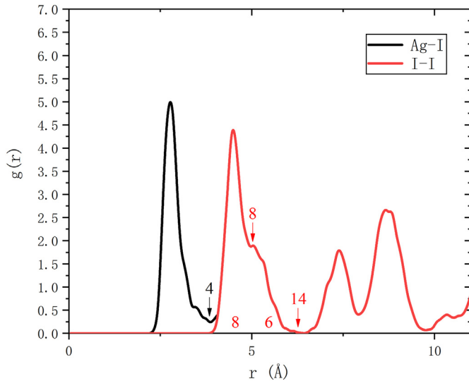
Fig. 12. The RDF at about 600 K obtained by heating the cooled system.
