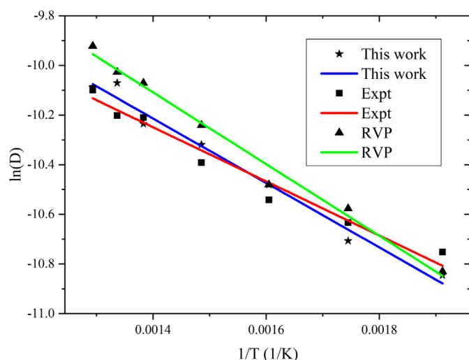
Fig. 9. The natural logarithm of \text{Ag}^+ diffusion coefficient (the symbol) versus the reciprocal of temperature: Arrhenius curve.
