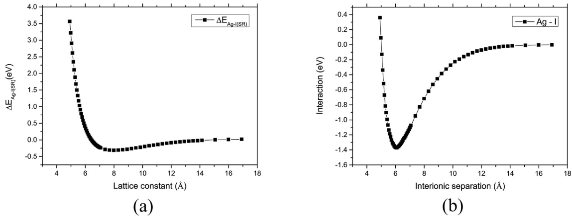
Fig. 3. (a) The short-range Ag-I interaction difference between B1- and B3-AgI versus lattice constant and (b) the short-range Ag-I pair potential versus interionic separation, which is derived from panel (a).
