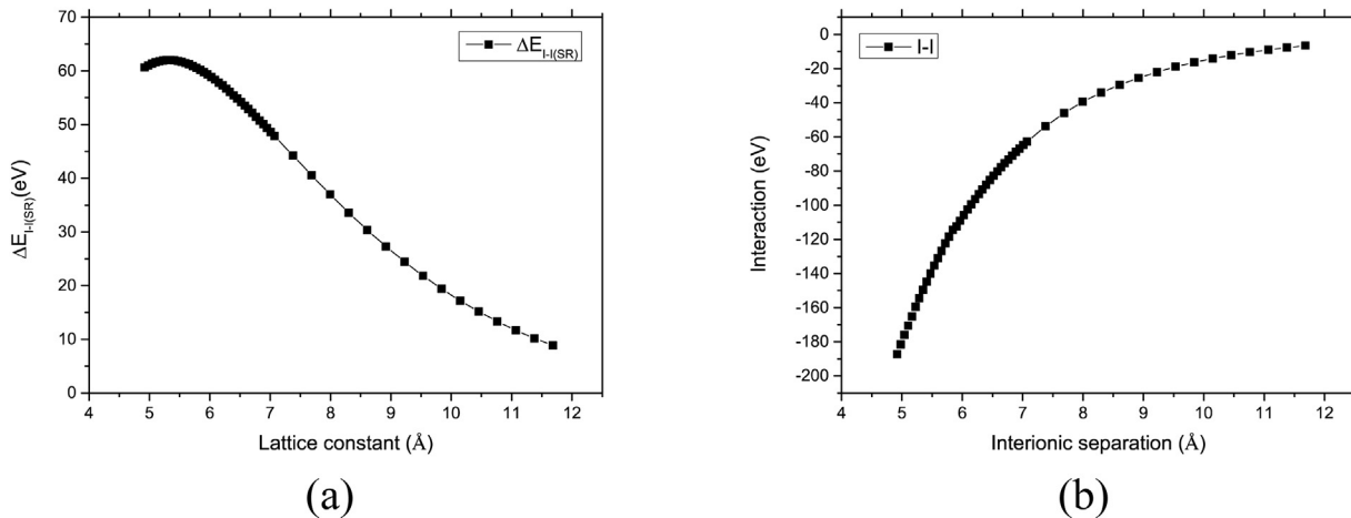
Fig. 4. (a) The short-range I-I interaction difference between B1- and T1-AgI versus lattice constant and (b) the short-range I-I pair potential versus interionic separation, which is derived from panel (a).
